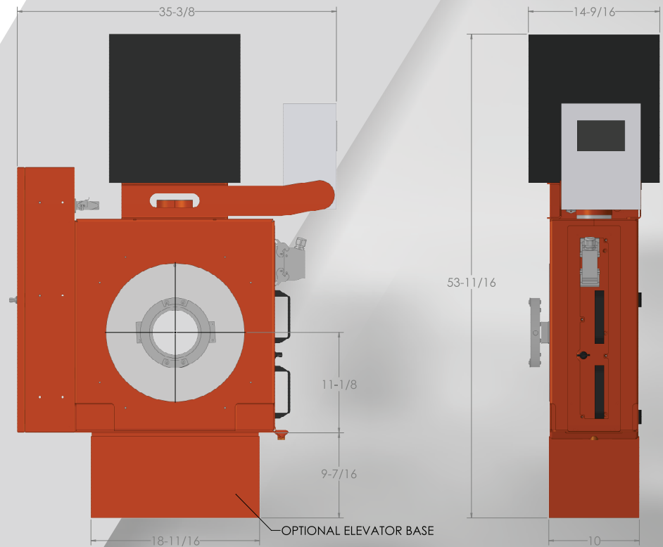
*DIMENSIONS SHOWN IN INCHES FOR ANTIRUST 04 AND 08
